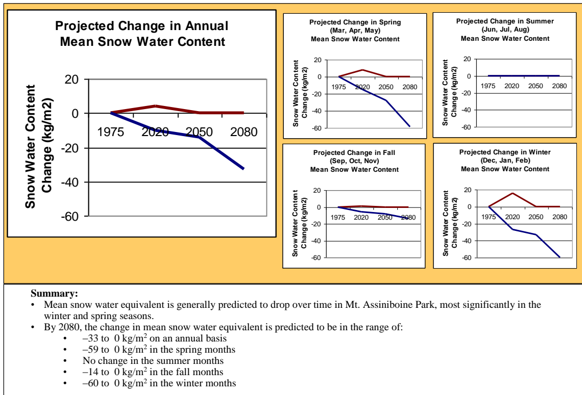
Figure 11: Projected change in mean snow water equivalent in Mt. Assiniboine Park
