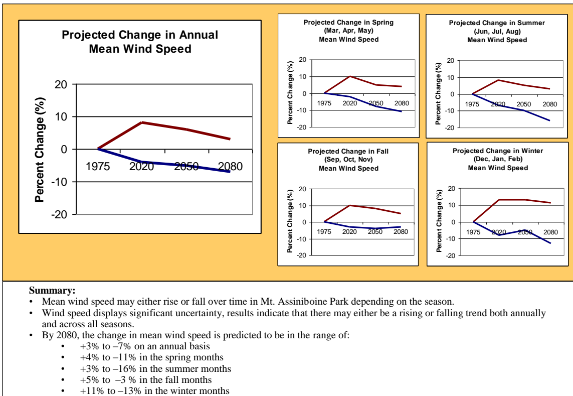
Figure 10: Projected change in mean wind speed in Mt. Assiniboine Park
