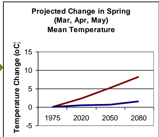
Figure 5: Example of simplified chart used for summary purposes. In this case, only the change is presented, therefore the 1975 point of reference is placed at zero. The upper and lower lines represent the highest and lowest possible scenario results at each time slice.
