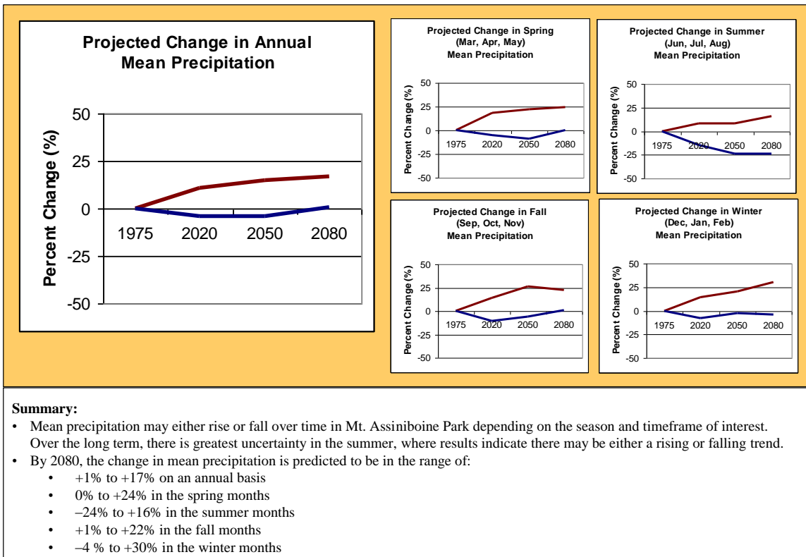
Figure 8: Projected change in mean precipitation in Mt. Assiniboine Park
