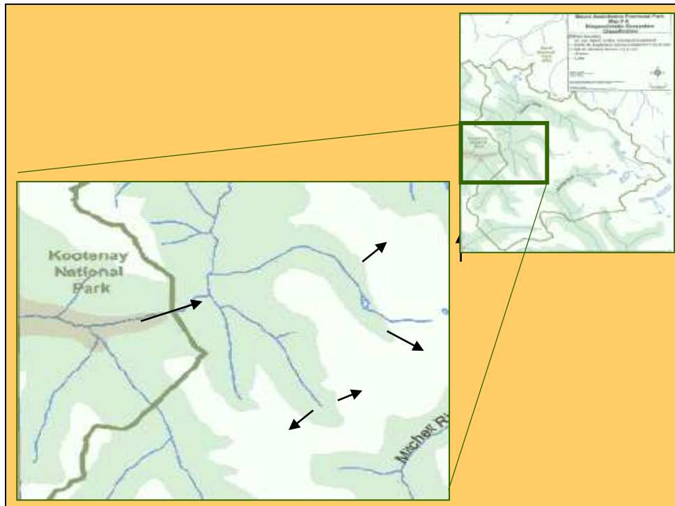
Figure 14: Conceptual Representation of Potential Expansion of ESSF and MS Zones
