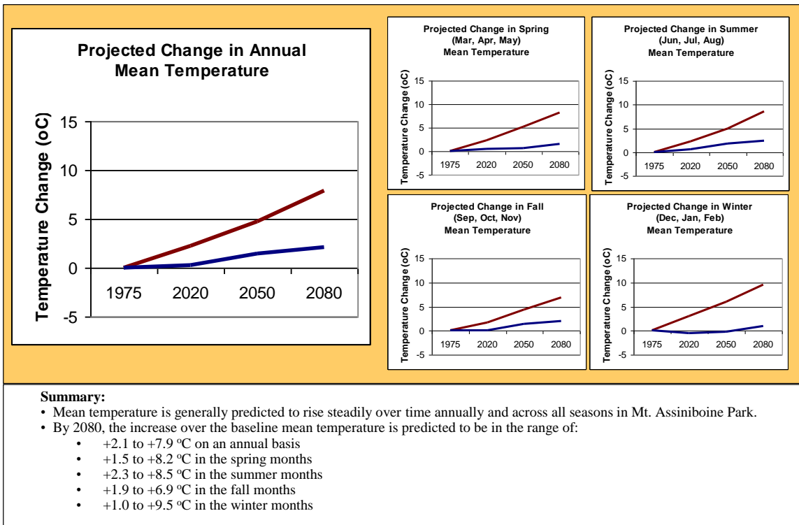
Figure 7: Projected change in mean temperature in Mt. Assiniboine Park
