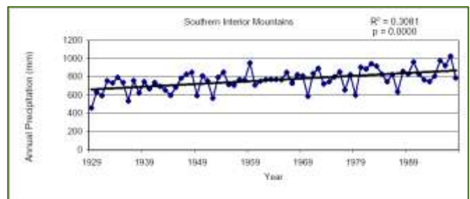
Figure 3: Historical trend in annual average precipitation for the Southern Interior Mountains Ecoprovince. Statistically significant at the 5% level.
