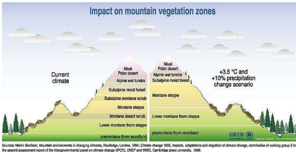
Figure 13: Conceptual diagram of shifting mountain vegetation zones
