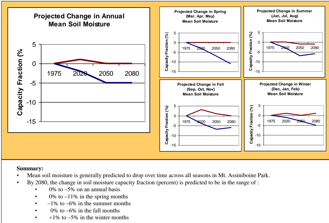
Figure 9: Projected change in mean soil moisture in Mt. Assiniboine Park
