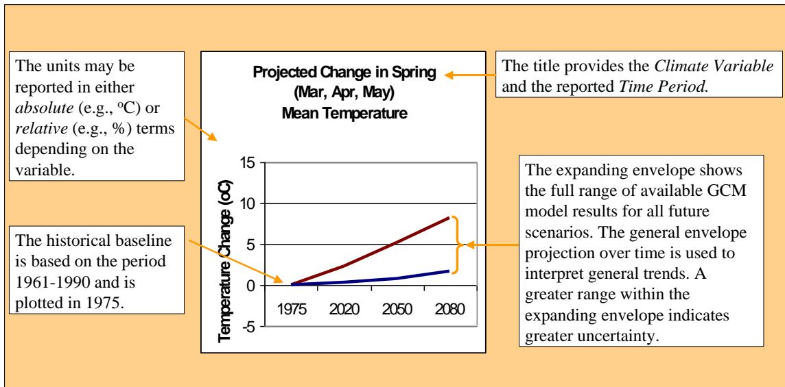
Figure 6: Interpretation of the climate projection envelope line charts
