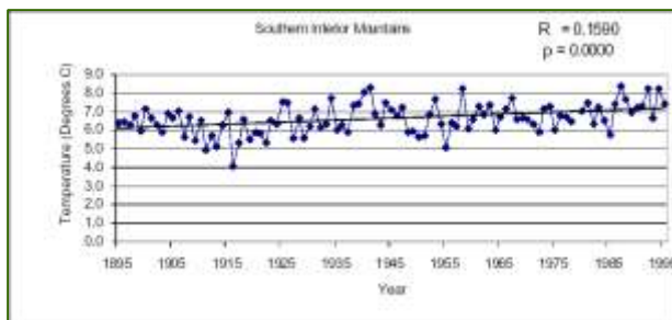
Figure 2: Historical trend in annual average temperature for the Southern Interior Mountains Ecoprovince. Statistically significant at the 5% level.
